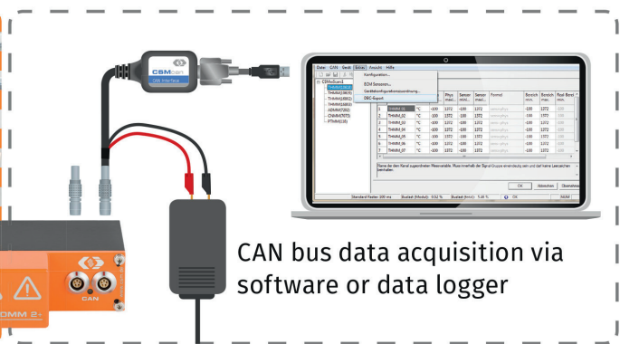
Typical measurement setup in a high-voltage environment using a CSM measurement system.
